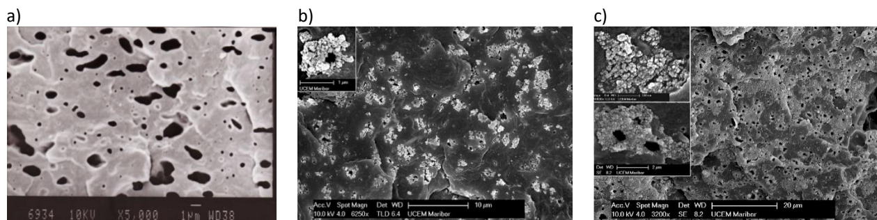
Figure 1: a) SEM pictures showing different morphologies: iPP/SEBS binary blend 80/20; b) iPP/silica 96/4 + 20% SEBS; c) iPP/silica 96/4 + 20% SEBS- g -MA
